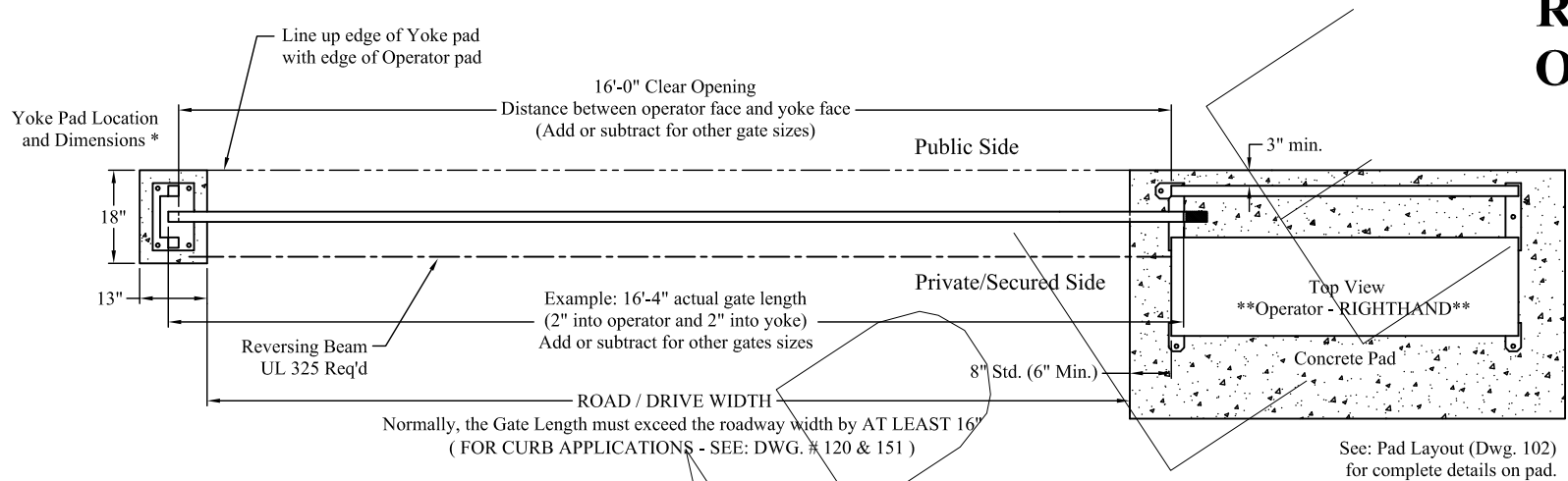
Example Shown: 16' x 5' Buckeye Style 500 Gate
