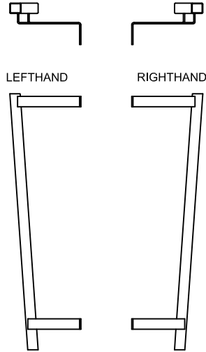
STYLE 'C' Offset Wall or Post Mounted
