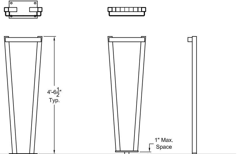
STYLE 'E' Standard Pad Mounted
