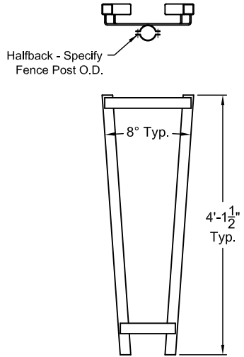
Grade STYLE 'A' Post Mounted
