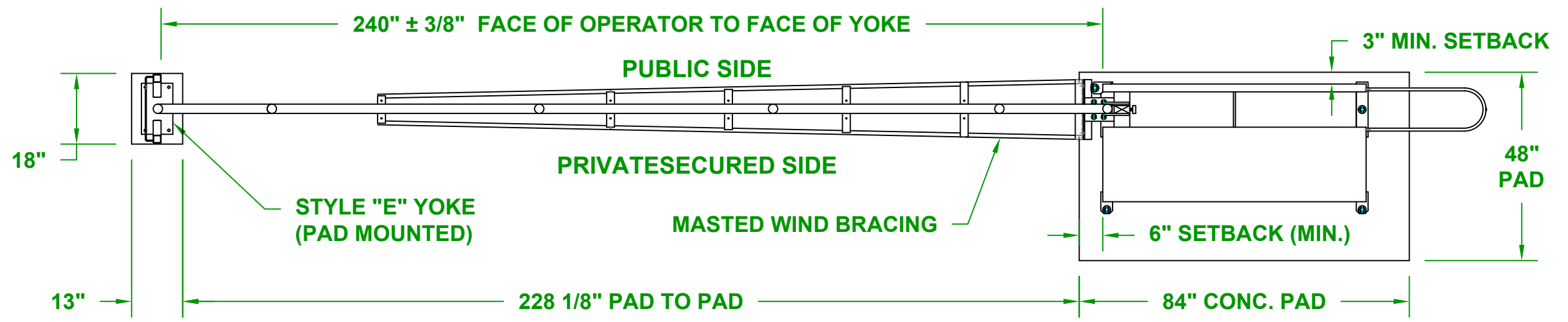
PLAN VIEW
