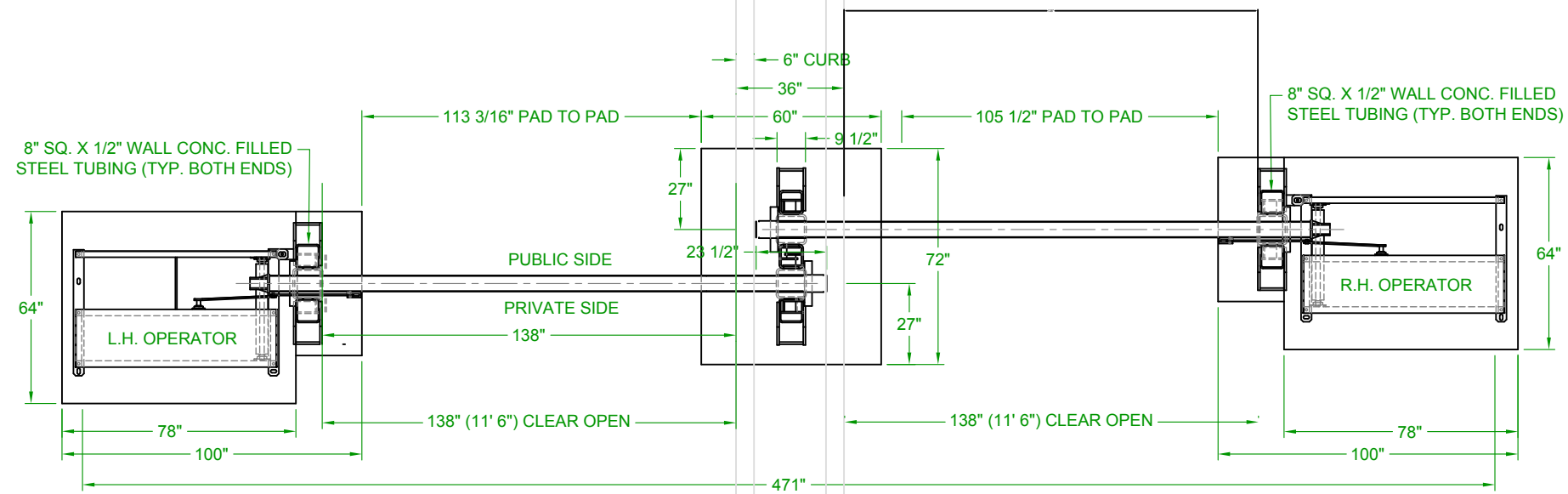
PLAN VIEW
