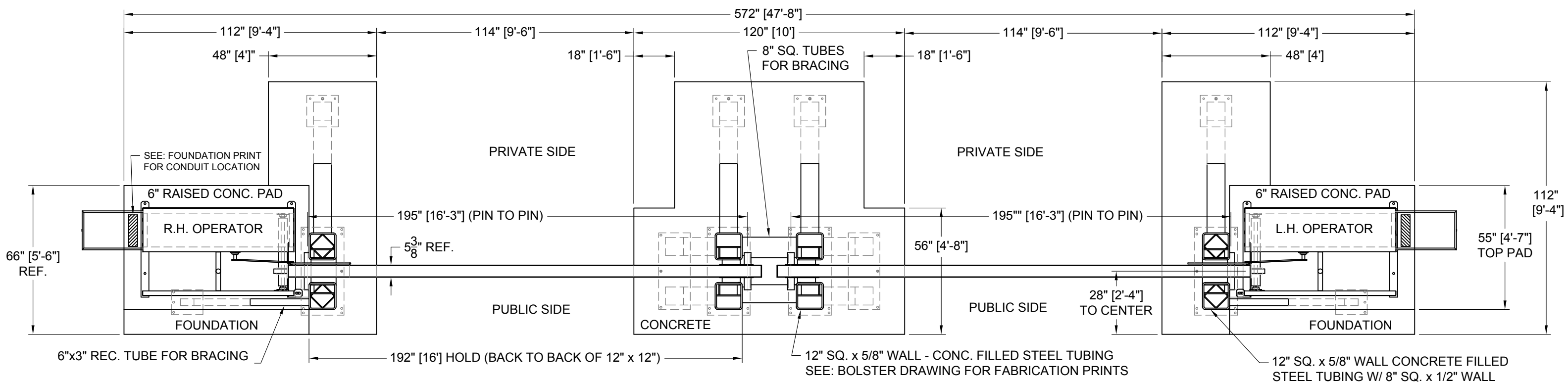
PLAN VIEW
