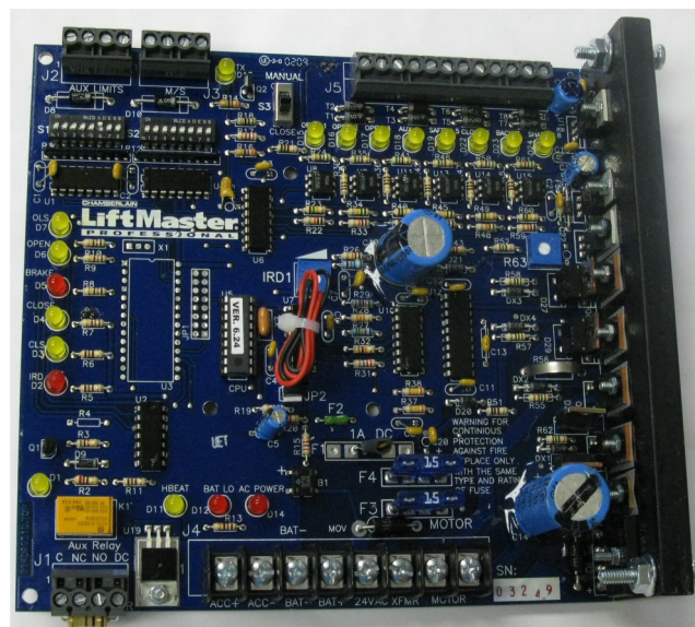
LiftMaster Control Board: Part # R-0128 (custom AutoGate Chip Ver. 6.24A)
