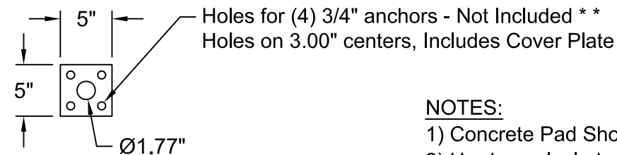
BASE PL. DETAIL
