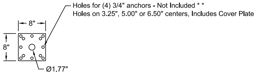
BASE PL. DETAIL
