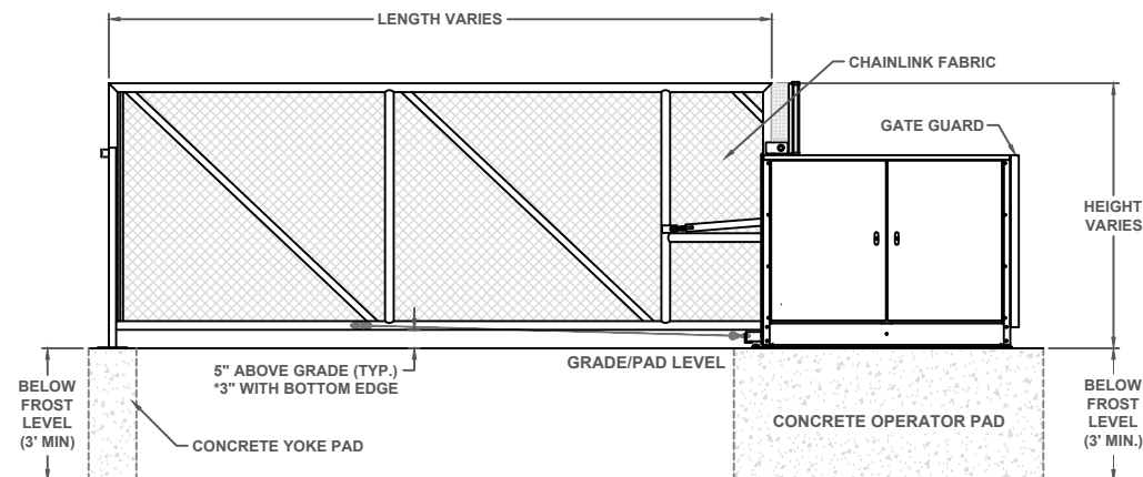
ELEVATION VIEW VIEWED FROM THE PRIVATE SIDE
