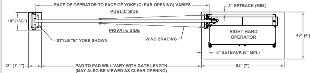
PLAN VIEW
